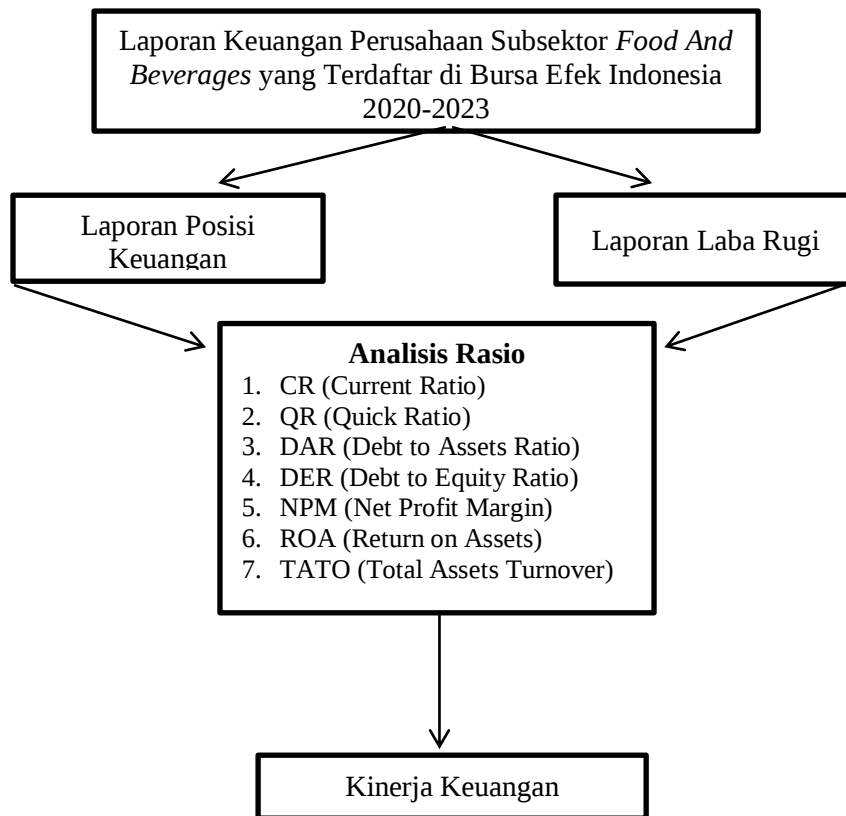
Gambar 2.1 Model Konseptual
